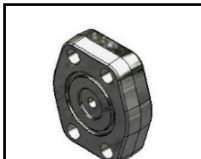
Blanking Flange O-Ring Face with Clearance Holes BR0104, BF0104M Page I16
