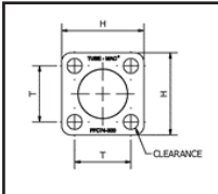
F10 Flare Flange Dimensions Metric Page K2
