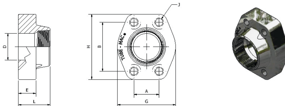
NTFF64 NPT Female Thread Flange - SAE Code 62 Flat Face with Threaded Holes
