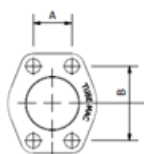
Retain Ring Flange Dimensions Page H25
