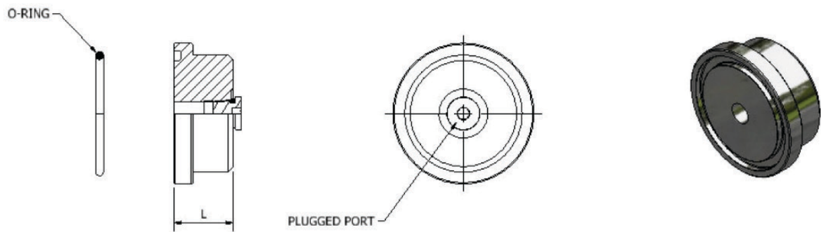
SFP64 - Complete with Buna O-Ring (Standard) and #4 SAE Port (Plugged), NPS
