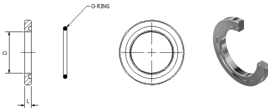
OSH – O-Ring Spacer for Retain Ring Pipe to Hose End
