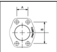
Retain Ring Flange Dimensions
