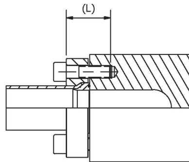
FLANGE TO COMPONENT
