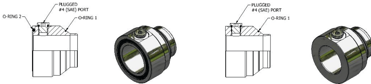
COP and CFP - Cone Inserts with Pilot Port for Flare Flange Connections, NPS
