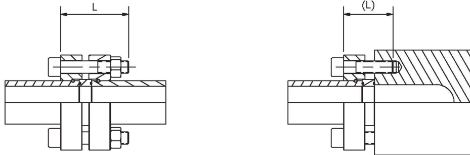
FLANGE TO FLANGE UNION
